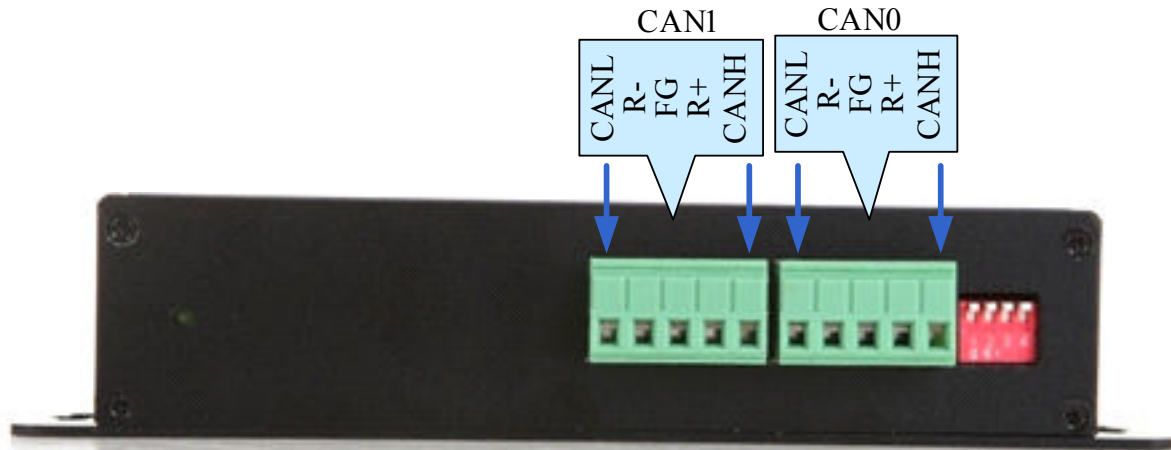
Figure 2-2-2-1 CAN Interface
