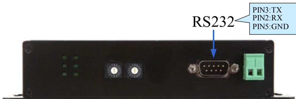
Figure 2-2-6-1 RS232 Interface
