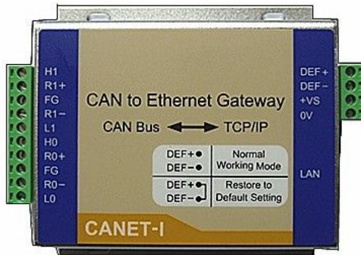
Figure 2-1 : CANET-I CAN interface module
