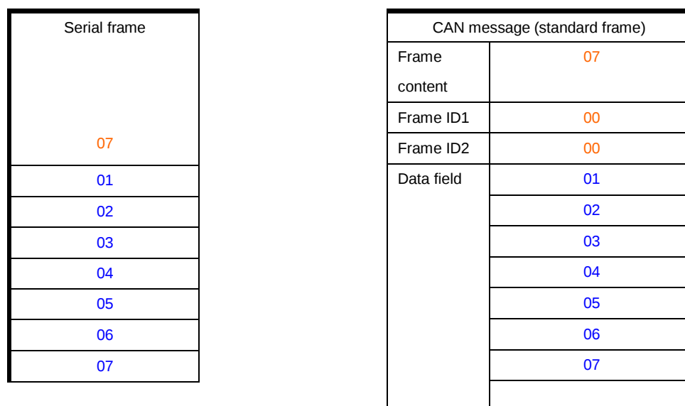
Figure 4.4 Example of converting CAN message to series frame (transparent mode)
