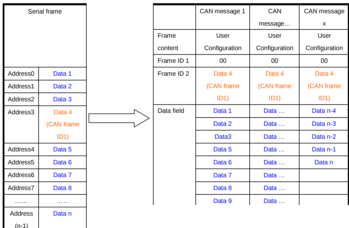
Figure 4.6 series frame converting to CAN message (transparent conversion with mark)
