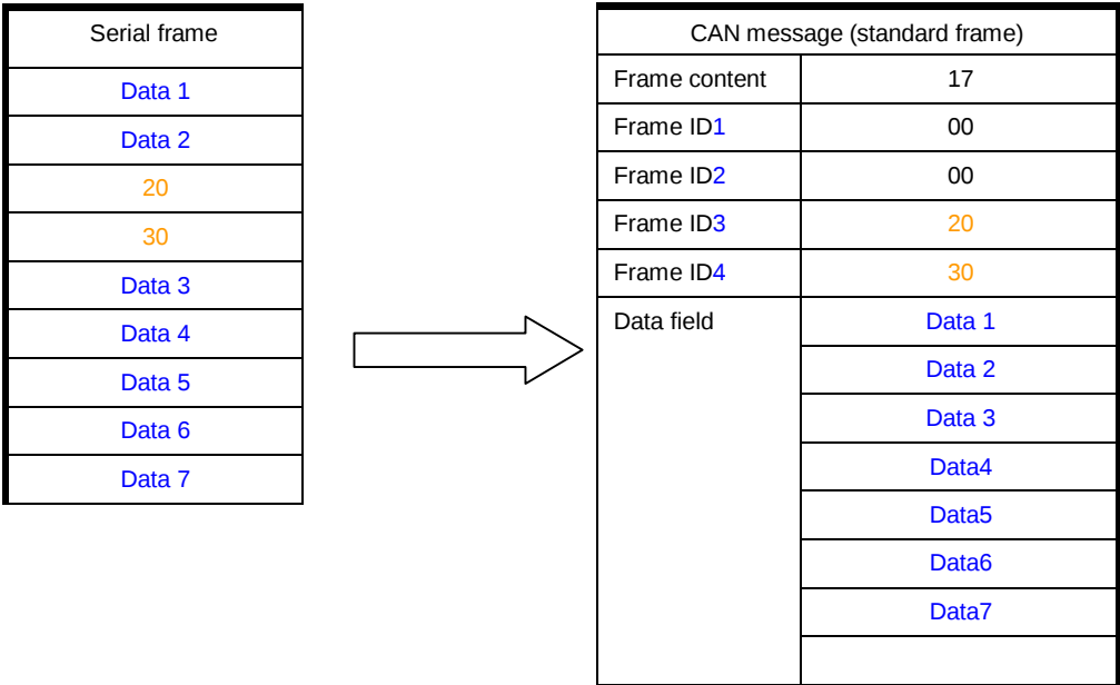
Figure 4.9 Example of converting CAM message to series frame (transparent conversion with mark mode)
