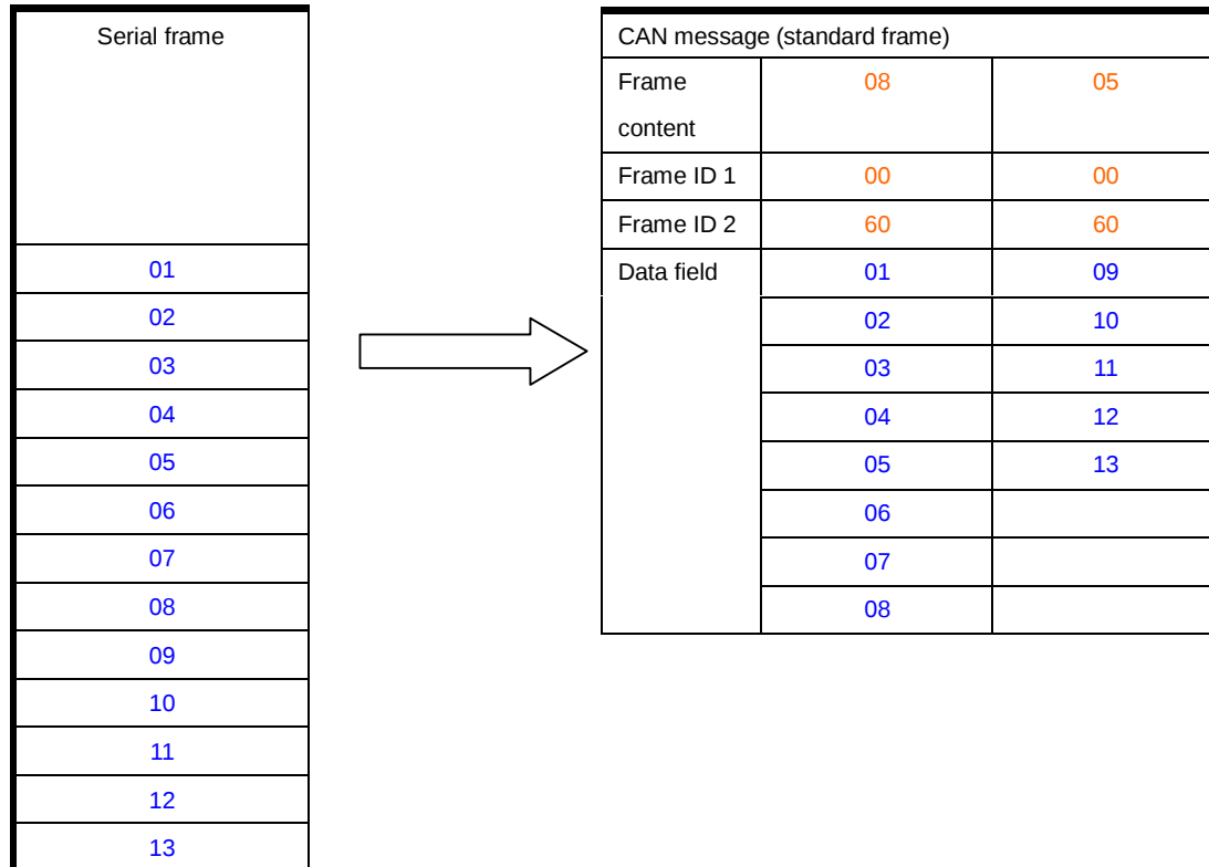
Figure 4.4 Example of converting CAN message to series frame (transparent mode)
